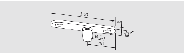
PT 24 pivot 15 mm Ø, with fixing plate, material thickness 6 mm, to let into ceiling Art. No. 01.116 Weight in kg: 0.058 aluminium
