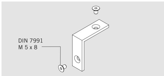
Corner connection set MR 28, 4 pieces per set
