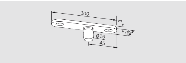
PT 24 pivot 15 mm Ø, with fixing plate, material thickness 3 mm, to screw on the ceiling Art. No. 01.123 Weight in kg: 0.042 aluminium stainless steel 0.074
