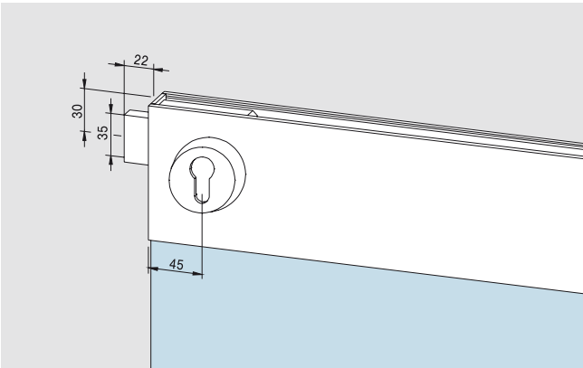
...with side locking lock, prepared for Europrofile cylinder, double throw 100 mm:
