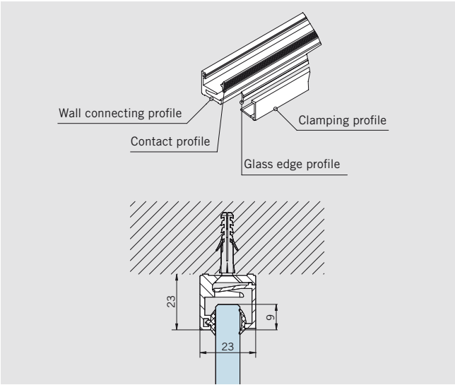
Base profile
