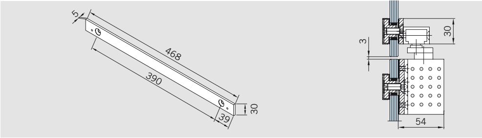
Fixing plate for DORMA TS 92, slide channel for overpanel Art. No. 12.332 Weight in kg aluminium 0.265
