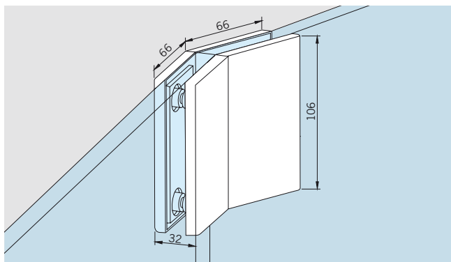
PT 80 connector, angle 135°
