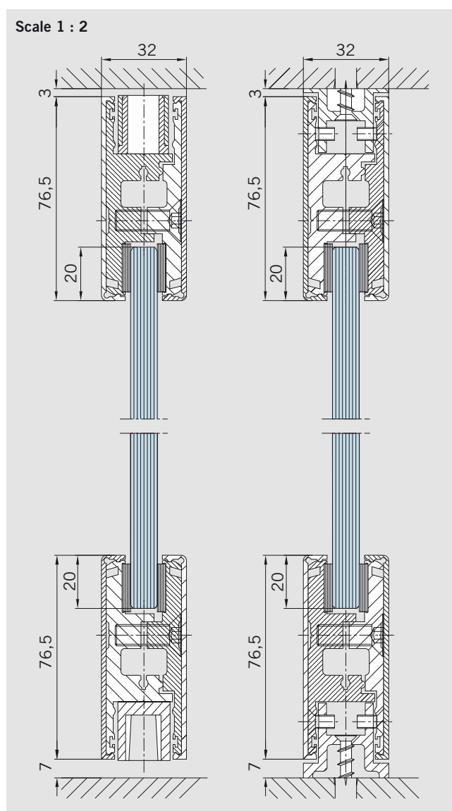
Door rails, 76.5 mm high
