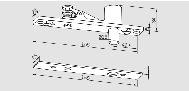
PT 21 frame portion top centre with removable pin 15 mm Ø, with cover plate Art. No. 01.118 Weight in kg: 0.345
