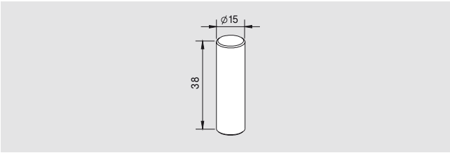
Loose pivot pin for interface between patch and rail Art. No. 04.601 Weight in kg: 0.050
