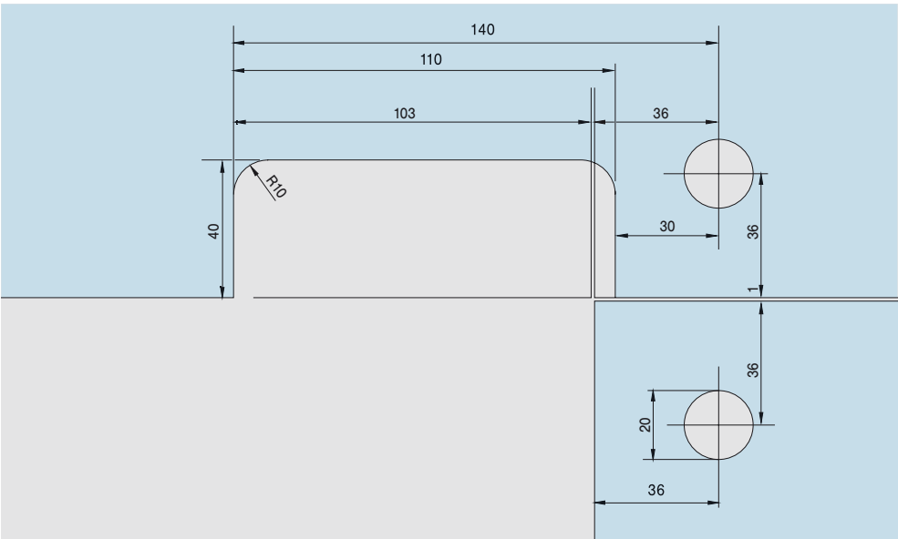
Undivided overpanel
