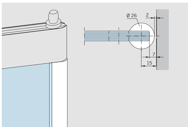
Radiused edging strip* for pinch free doors, (strip is clamped onto free glass edge), acrylic. Length: up to 4500 mm (please specify height)
