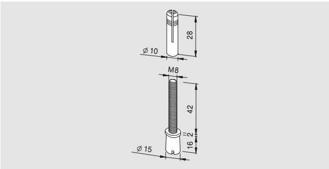
PT 25 pivot 15 mm Ø with plug Art. No. 01.115 Weight in kg: 0.044
