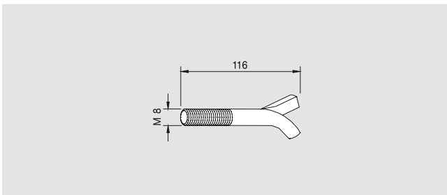
Wall anchor with thread M 8 for overpanel patch
