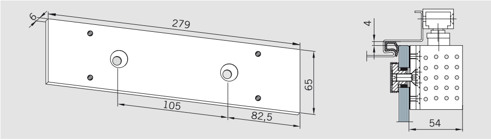
Fixing plate 279 mm, for DORMA TS 92 Art. No. 12.334 Weight in kg: aluminium 0.290
