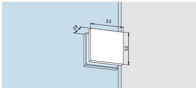
PT 90 Srew on fitting
