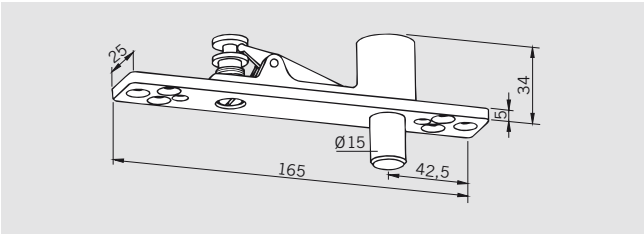
PT 21 frame portion top centre with removable pin 15 mm Ø Art. No. 01.117 Weight in kg: 0.335
