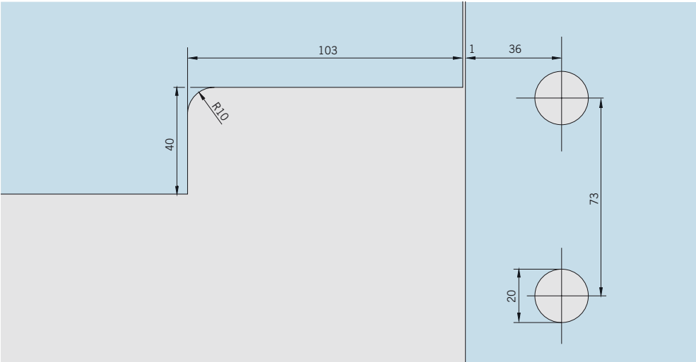
Divided overpanel
